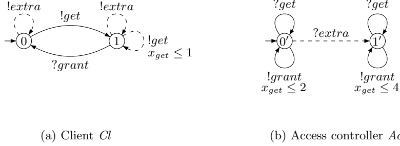
Fig. 2. Client Cl and access controller Acc
