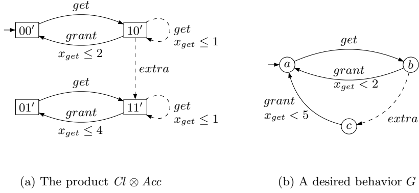
Fig. 3. The global model Cl \otimes Acc and its specified behavior G
